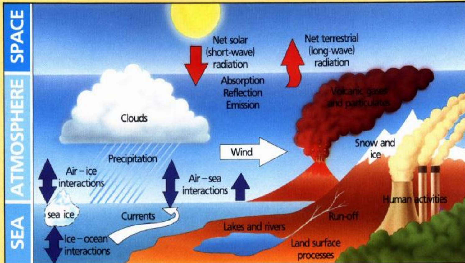
The Climate System
