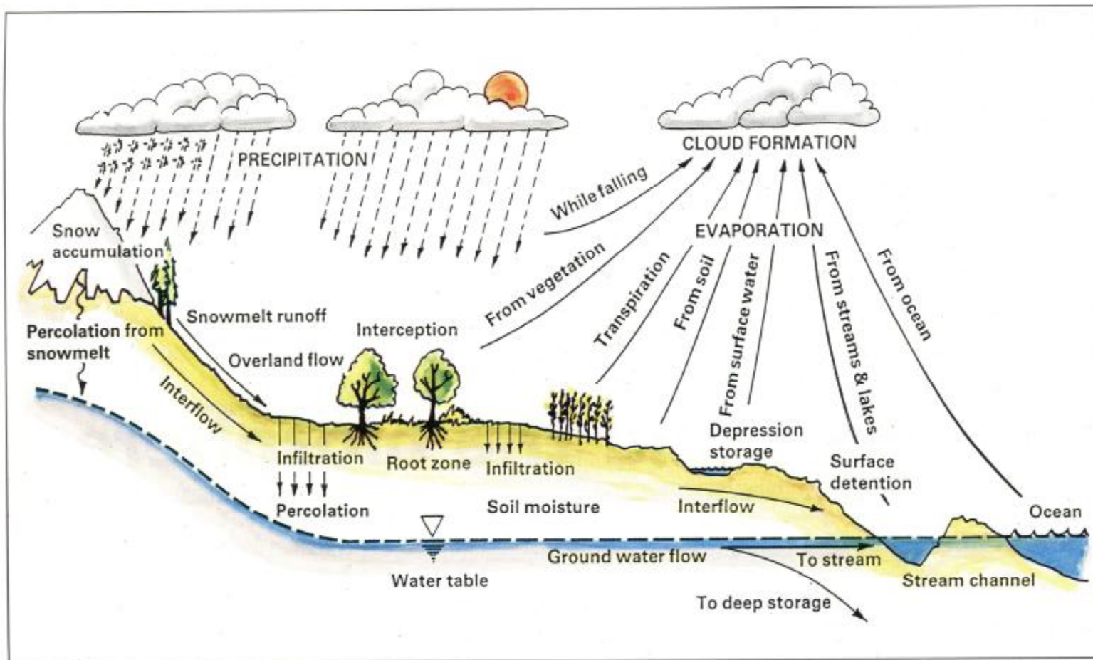
Figure 1 Circulation of water through the hydrological cycle (National Aeronautics and Space Administration, 1984)
